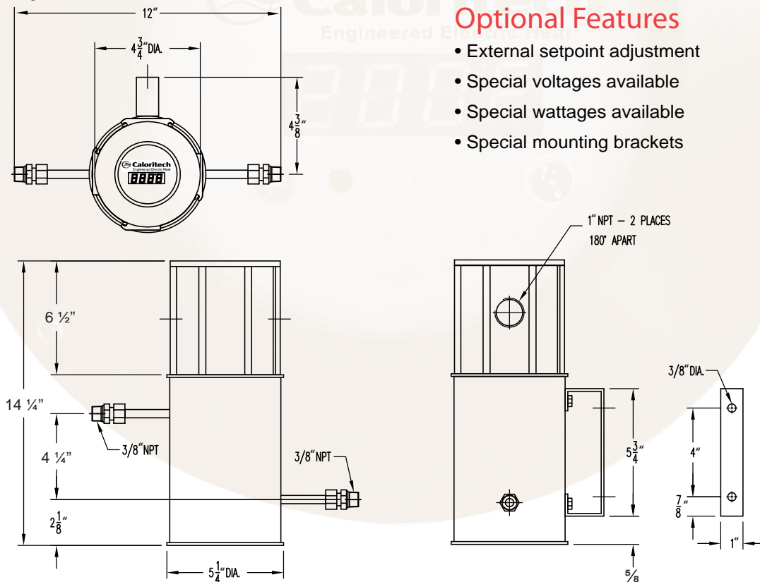
Figure 1 - Heater Dimensions
